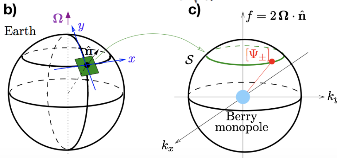
b and c–We explained the Existence of two unidirectional modes filling the frequency gap, computing inertia-gravity waves in a plane tangent to the Earth and showed that they carry a Chern number of value 2 in parameter space.
